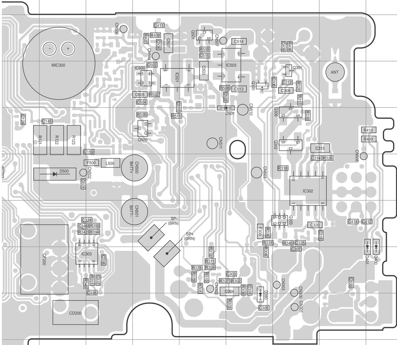
TX-RX UNIT (X57-8092-71) Component side view (J79-0362-29)
