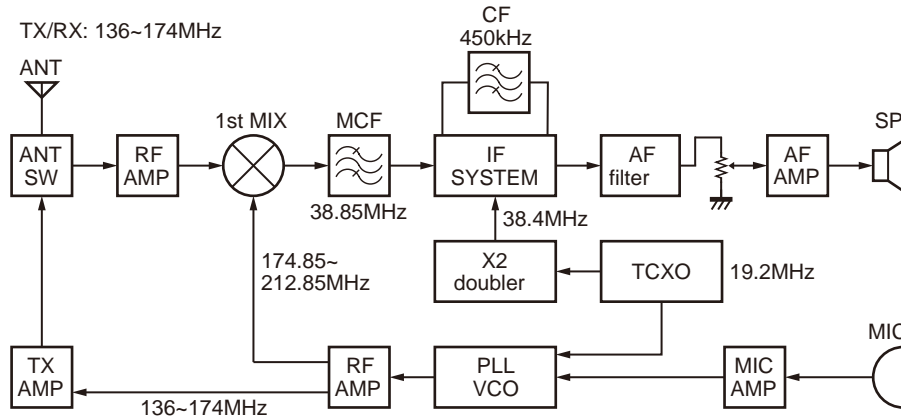
Fig. 1 Frequency configuration
