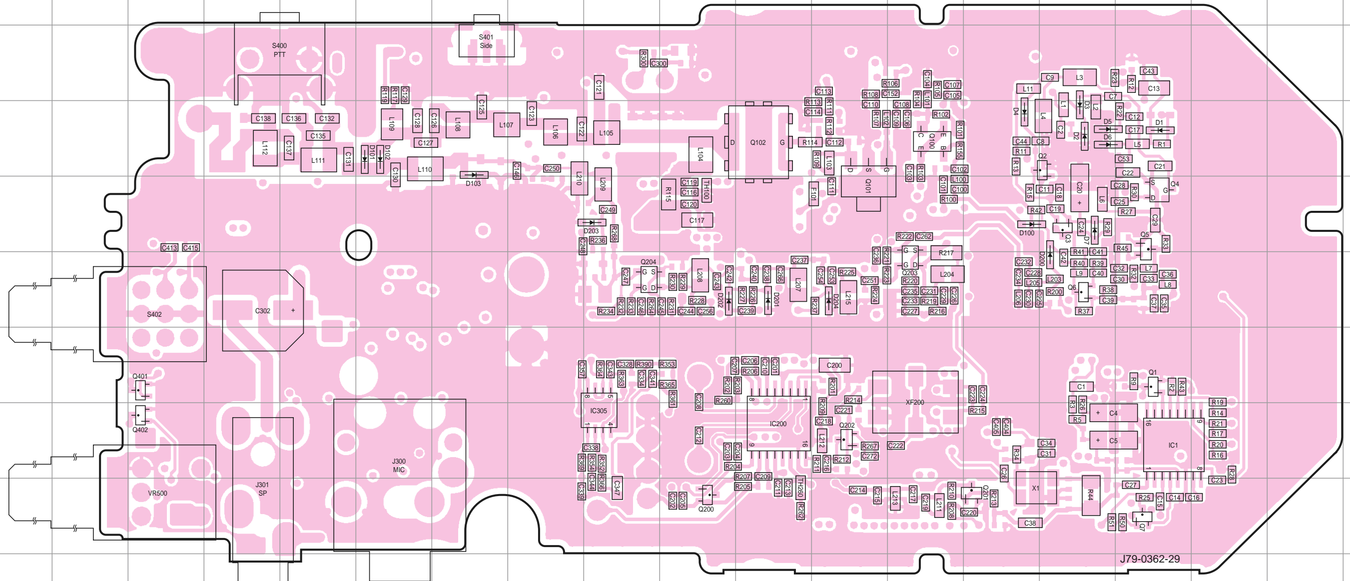
TX-RX UNIT (X57-8092-71) Foil side view (J79-0362-29)
