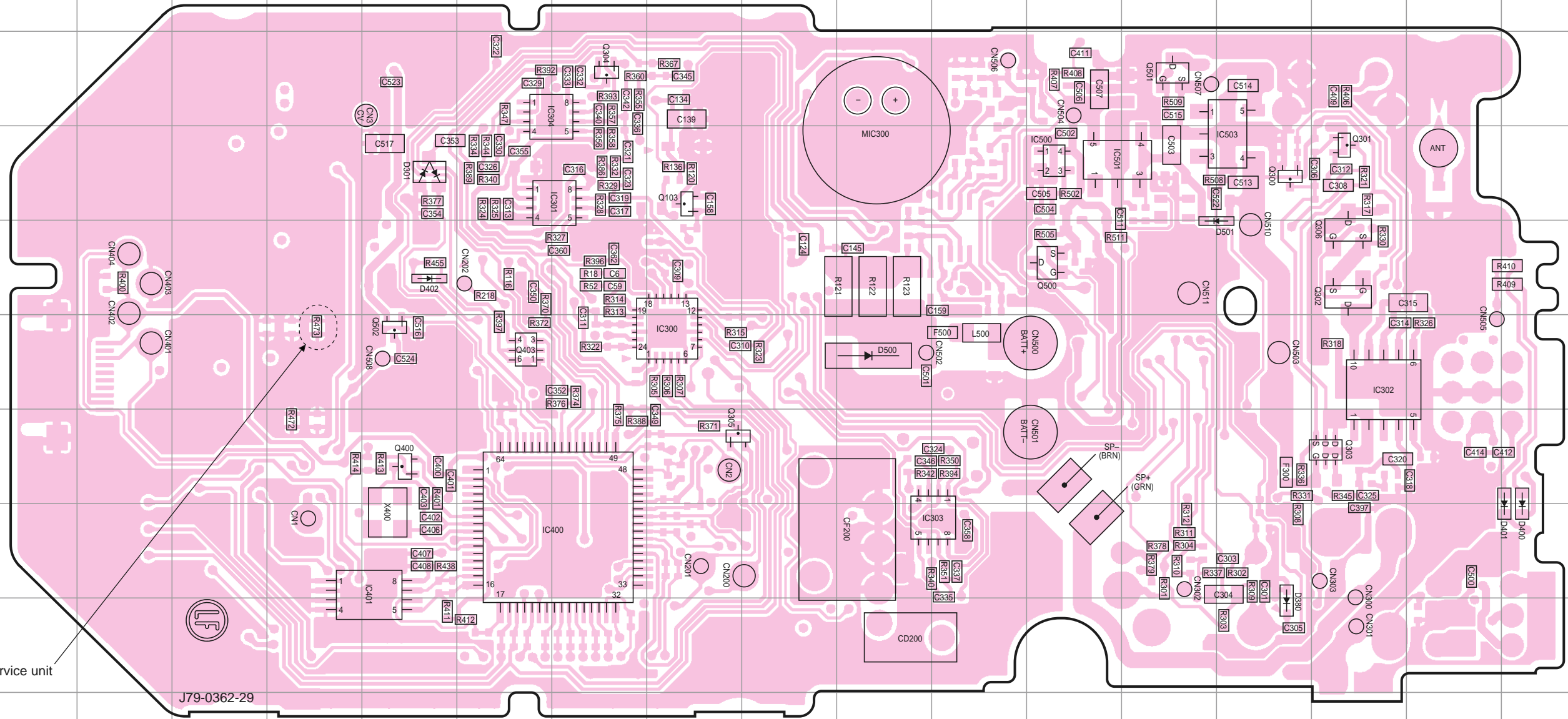
TX-RX UNIT (X57-8092-71) Component side view (J79-0362-29)
